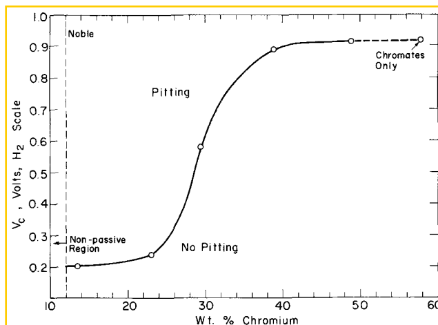
Fig. 1. Critical pitting potentials for Cr-Fe alloys in 0.1N \text{NaCl} , 25^\circ\text{C}
