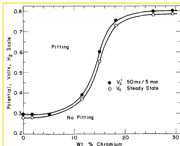
Fig. 2. Critical pitting potentials for Cr-Ni alloys in 0.1N \text{NaCl} , 25^\circ\text{C}
