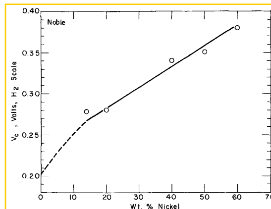
Fig. 5. Critical pitting potentials for 15% Cr-Fe alloys with increasing Ni content, in 0.1N NaCl, 25°C.
